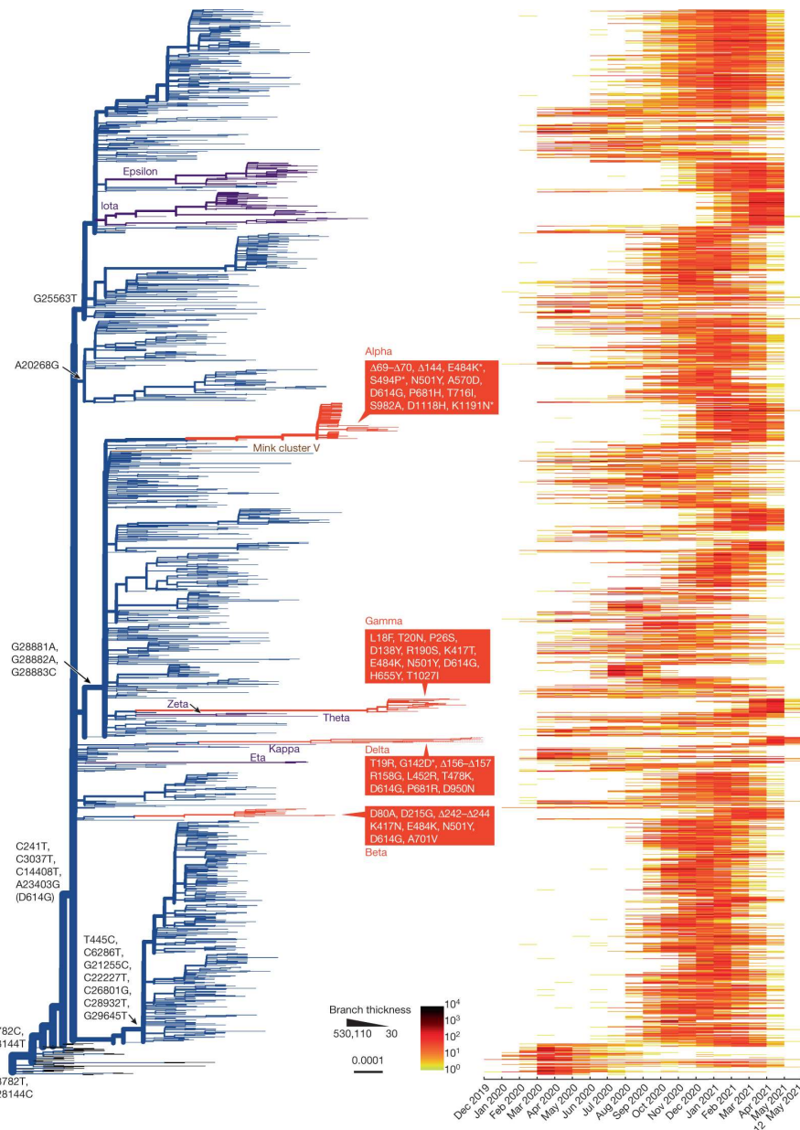
Figure showing Phylogenetic tree of SARS-CoV-2 lineages and the temporal distribution of major sequence variants.
